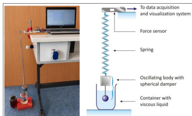
Fig 1: Photograph and diagram of the experimental apparatus used to study oscillations during the instructional intervention
