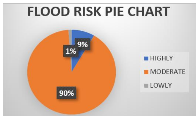
Fig 13: Showing the pie chart of the flood risk
