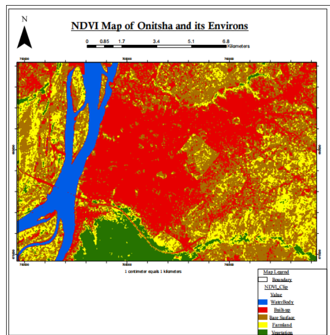
Fig 11: Showing NDVI Map after reclassification
