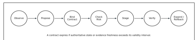
Fig 2: Contract lifecycle. Authorization is repeated when authoritative state changes or the contract expires
