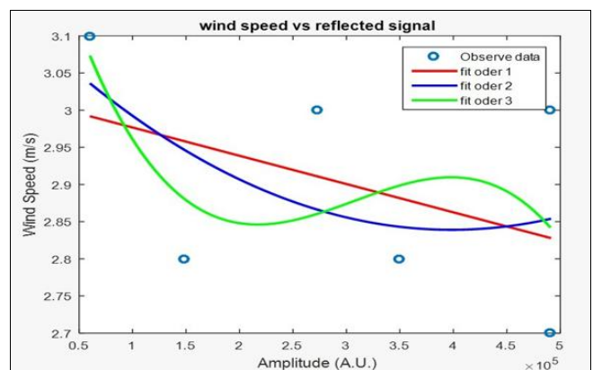
Fig 7: Wind speed versus amplitude in different order fitting
