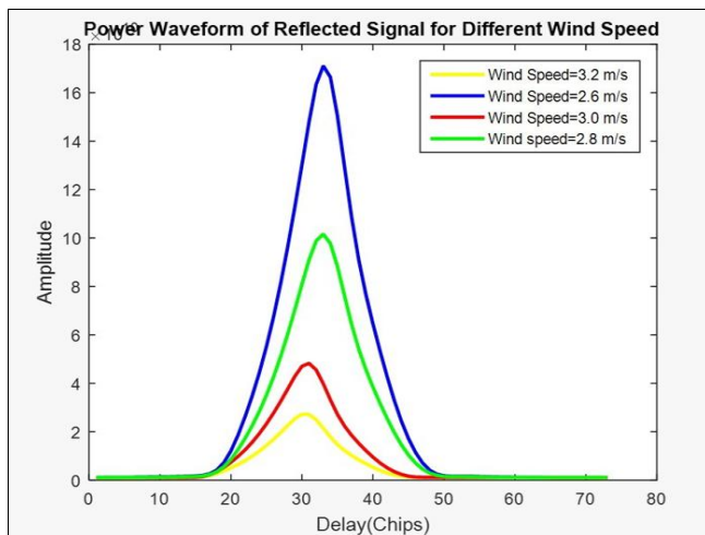
Fig 4: Power waveforms of reflected signals for different wind speed
