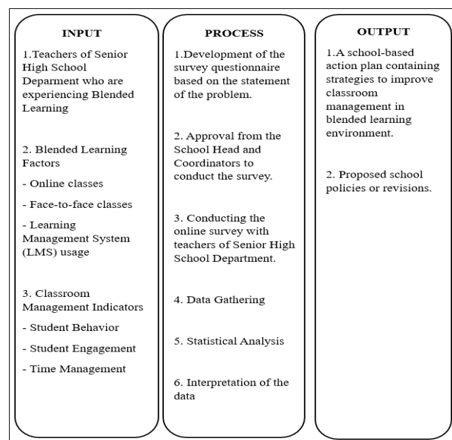
Fig 1: Input-Process-Output Model
