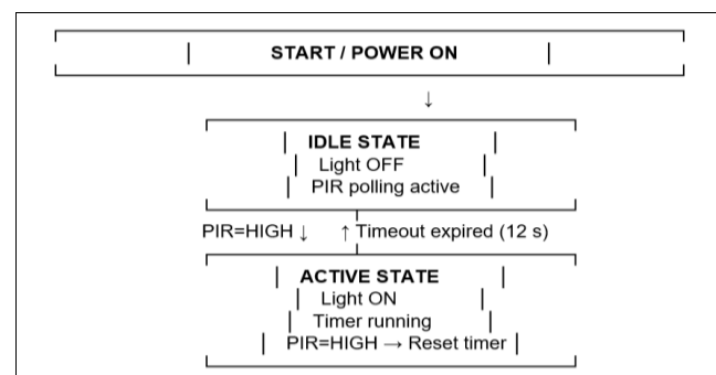
Fig 3: Finite-State Machine (FSM) Diagram of the Motion-Responsive Illumination System
