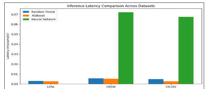
Fig 3: Inference latency comparison (ms per sample) of Random Forest, XGBoost, and Neural Network models across different datasets
