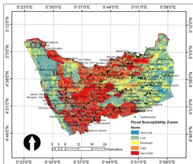
Fig 1: Flood Susceptibility Zones in Ekeremor LGA
