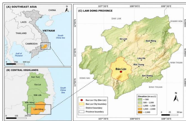
Fig 1: Location of the study area in Bao Loc City (Lam Dong Province), Central Highlands of Vietnam
