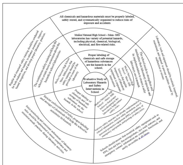
Fig 1: Web Scheme
