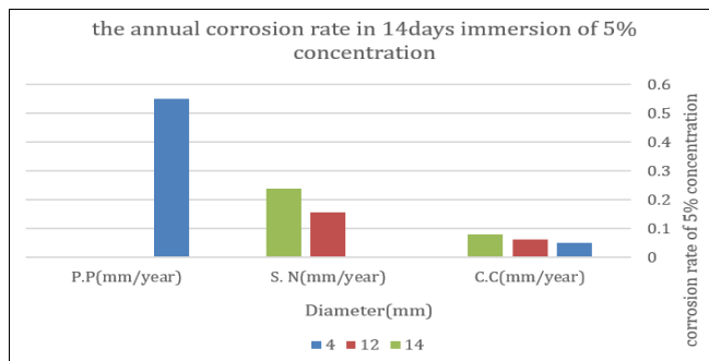
Fig 7: The annual corrosion rate in 14 days immersion of 5% concentration of (Calcium Carbonate C.C, Sodium Nitrate S.N, and potassium phosphate P.P)
