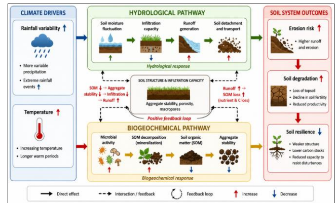
Fig 2: Process-based conceptual model illustrating coupled hydrological-biogeochemical interactions under climate variability in tropical agroecosystems
