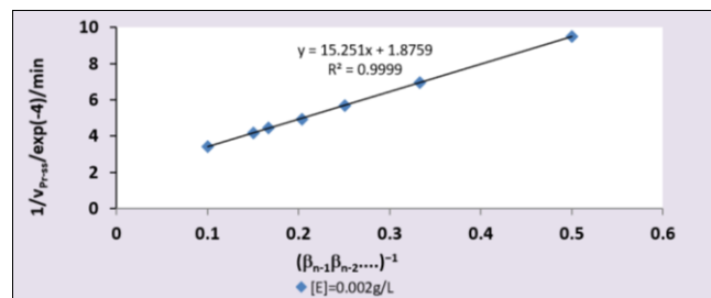
Fig 6: The reciprocal of initial rates as a function of the product of the ratio of substrate concentrations where the concentrations of the enzyme is 0.002 \text{ g/L} . Note that taking the reciprocal of the slope (which is k_{cat} ) divide by [S_T]_1 (the first substrate concentration in the range) and multiplying by the molar concentration of the enzyme gives \approx 8.41 \text{ exp. (-5) mol./g min} .
