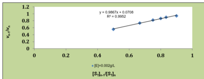
Fig 3: The ratio of initial rates as a function of the ratio of the corresponding concentration of the substrate, plotted versus the latter where [E_0] = 0.002 \text{ g/L} . [S_T]_n > [S_T]_{n-1} and v_{n-1} < v_n where n is the number of assays (or “population size”) for the initial rates, v , and concentrations of the substrate
