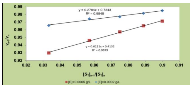
Fig 4: The ratio of initial rates as a function of the ratio of the corresponding concentration of the substrate, plotted versus the latter where [E_0] = 0.0002 \text{ g/L} (◆) and 0.0005 \text{ g/L} (■)
