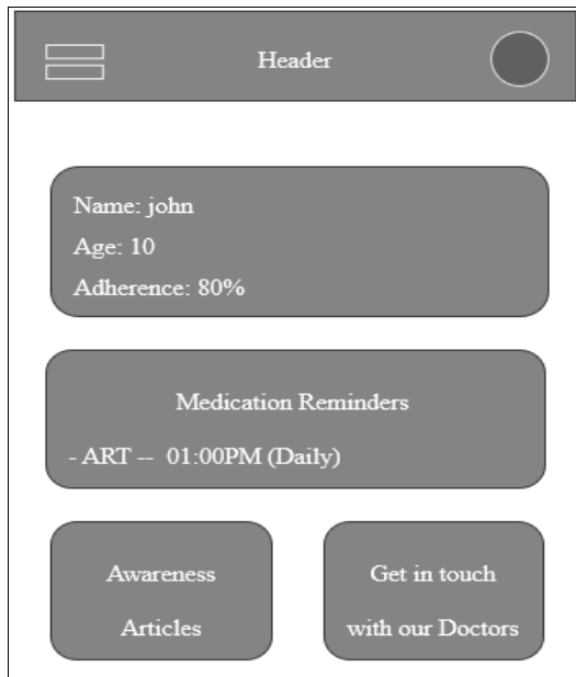
Fig 5: User interface
