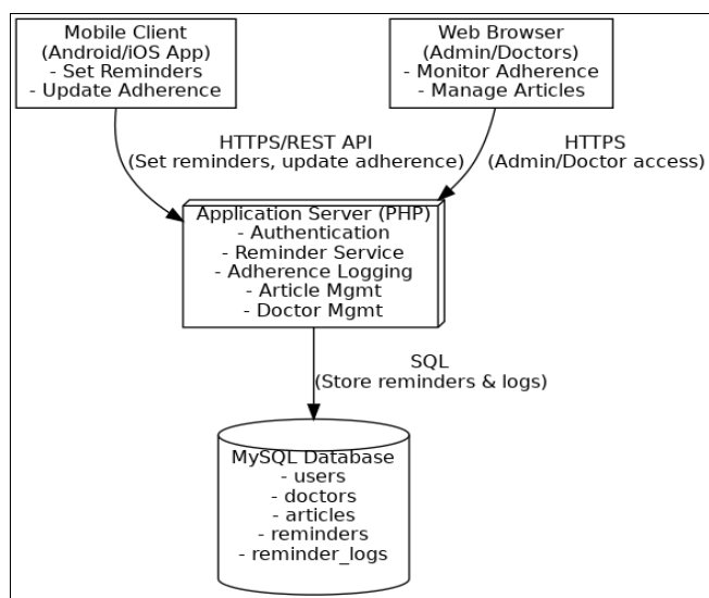
Fig 3: Client-server architecture
