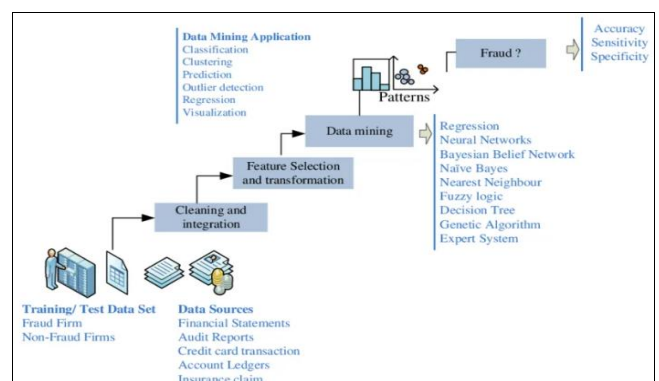
Fig 3: Data mining based framework for financial fraud detection (Barman, et al. , 2016)
