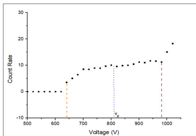
Fig 2: Geiger Plateau for determination of operating voltage
