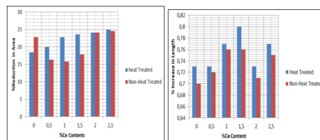
(a) Percentage Reduction in Area (b) Percentage Increase in Length
