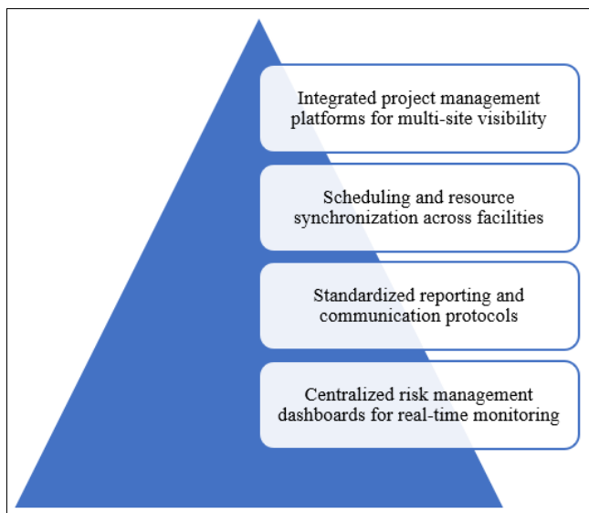
Fig 3: Coordination Mechanisms
