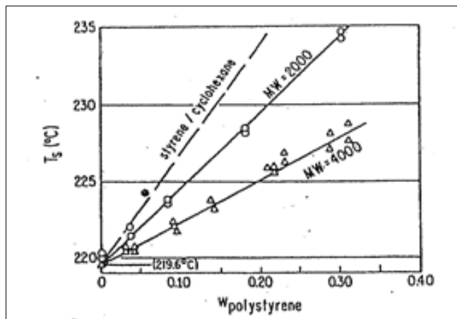
Fig 2: Data on limiting superheat for low molecular weight polystyrene in cyclohexane. T_s for pure cyclohexane is taken as 219.6^\circ\text{C} .
