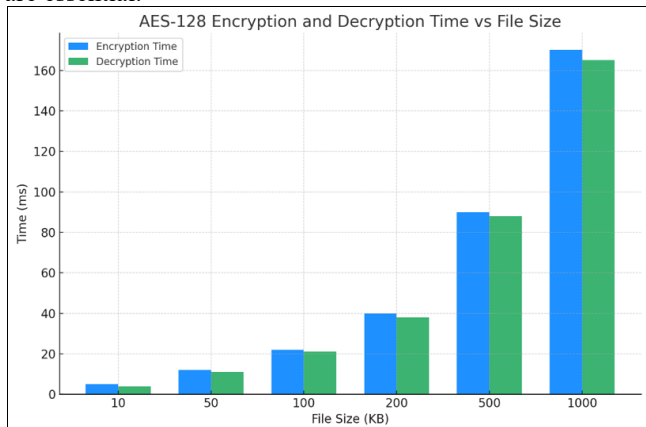
Fig 3: AES-128 Encryption and Decryption Time vs File Size
