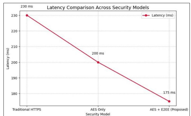
Fig 2: Latency Comparison Across Security
