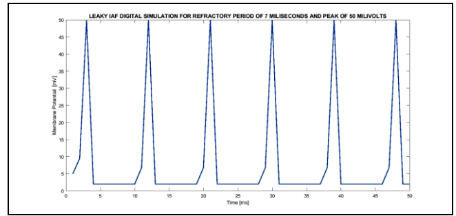
Fig 4: - 2D LIAF simulation, Input Intensity, Firing rate, and Threshold Potential. Almost exact simulation. Dataset for programming patterns: ( I_s = 5 \text{ nA} , C_m = 1 \text{ nF} , R_m = 10 \text{ M}\Omega , and T_{ref} \approx 7 \text{ ms} ; ( V_{th} = 10 \text{ mV} , V_{spike} = 50 \text{ mV} , simulation time 50 ms)). Note: the program is designed in splines, so the totally exact points at graph differ something in magnitude. [Casesnoves Bioengineering Laboratory Software 16.27].
