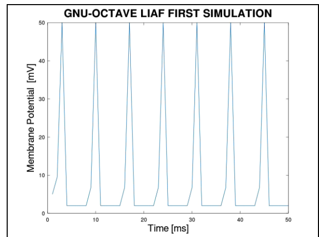
Fig 1.1: -GNU-Octave 2D LIAF simulation, Input Intensity, Firing rate, and Threshold Potential. Almost exact simulation. Dataset for programming patterns: ( I_s = 5 \text{ nA} , C_m = 1 \text{ nF} , R_m = 10 \text{ M}\Omega , and T_{ref} \approx 5 \text{ ms} ; ( V_{th} = 10 \text{ mV} , V_{spike} = 50 \text{ mV} , simulation time 50 ms)). Note: the program is designed in splines, and that makes some small image precision bias
