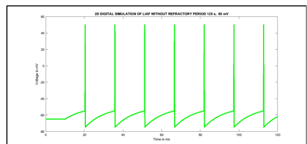
Fig 10: - 2D digital simulation for LIAF model without refractory period: ( I_s = 1.55 nA, R_m = 10 M \Omega , and ( V_{th} = 10 mV, V_{spike} = 50 mV, V_{reset} = 75 mV, simulation time 120 ms)). [Casesnoves Bioengineering Laboratory Software 16.33].
