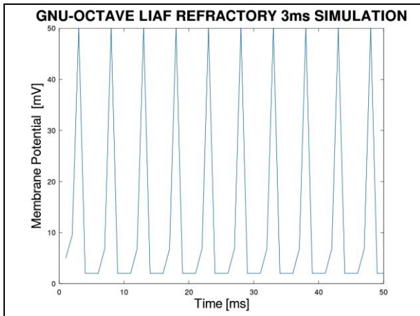
Fig 3.1: - GNU-Octave 2D LIAF simulation, Input Intensity, Firing rate, and Threshold Potential. Almost exact simulation. Dataset for programming patterns: ( I_s = 5 \text{ nA} , C_m = 1 \text{ nF} , R_m = 10 \text{ M}\Omega , and T_{ref} \approx 3 \text{ ms} ; ( V_{th} = 10 \text{ mV} , V_{spike} = 50 \text{ mV} , simulation time 50 ms)). Note: the program is designed in splines, so the totally exact points at graph differ something in magnitude. [Casesnoves Bioengineering Laboratory Software 16.26].
