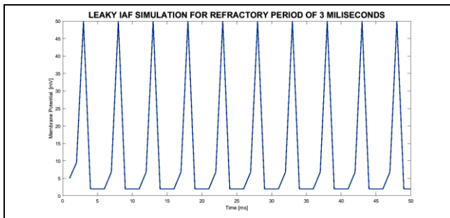
Fig 3:- 2D LIAF simulation, Input Intensity, Firing rate, and Threshold Potential. Almost exact simulation. Dataset for programming patterns: ( I_s = 5 \text{ nA} , C_m = 1 \text{ nF} , R_m = 10 \text{ M}\Omega , and T_{ref} \approx 3 \text{ ms} ; ( V_{th} = 10 \text{ mV} , V_{spike} = 50 \text{ mV} , simulation time 50 ms)). Note: the program is designed in splines, so the totally exact points at graph differ something in magnitude. [Casesnoves Bioengineering Laboratory Software 16.26].
