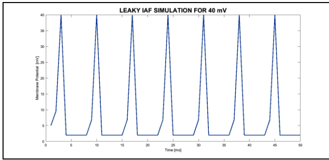
Fig 2:- 2D LIAF simulation, Input Intensity, Firing rate, and Threshold Potential. Almost exact simulation. Dataset for programming patterns: ( I_s = 5 \text{ nA} , C_m = 1 \text{ nF} , R_m = 10 \text{ M}\Omega , and T_{ref} \approx 4 \text{ ms} ; ( V_{th} = 10 \text{ mV} , V_{spike} = 40 \text{ mV} , simulation time 50 ms)). Note: the program is designed in splines, so the totally exact points at graph differ something in magnitude. [Casesnoves Bioengineering Laboratory Software 16.25].
