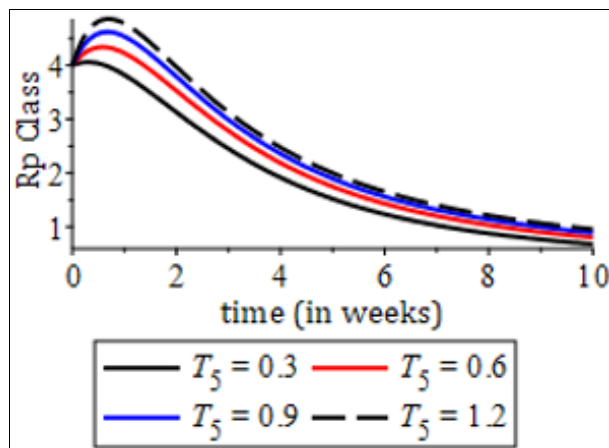
Fig 19: Impact of recovery rate with treatment to partial immunity on partial recovery class
