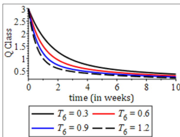
Fig 21: Impact of recovery rate with treatment to full immunity on quarantine class
