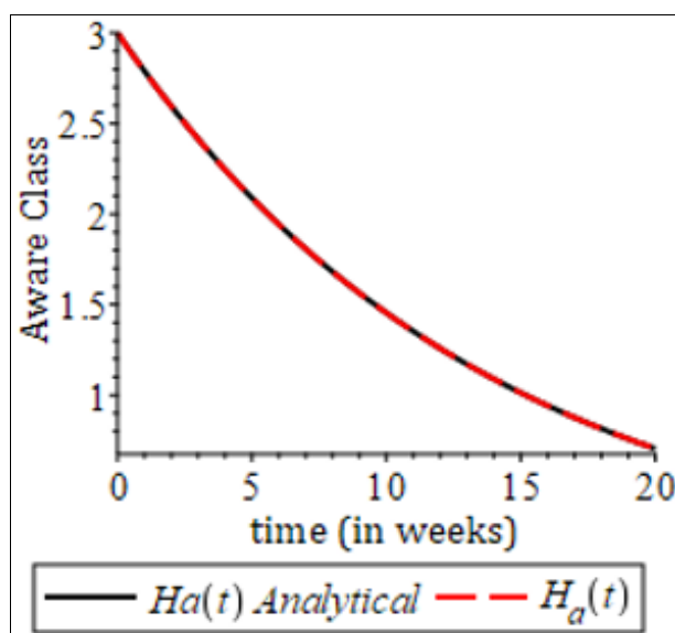
Fig 2: Comparison between Analytical (solid black line) and Numerical (dash red line) solution for aware class ( H_a(t) )
