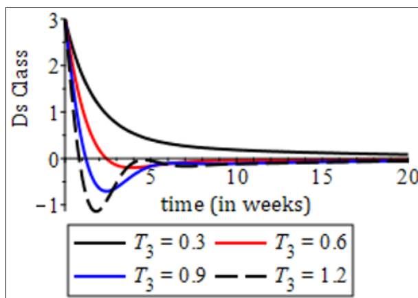
Fig 11: Impact of Isolation rate on symptomatically infected population
