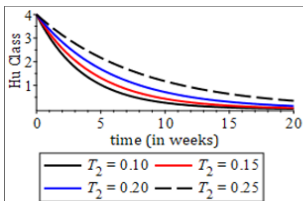
Fig 15: Influence of latency rate on Hu class
