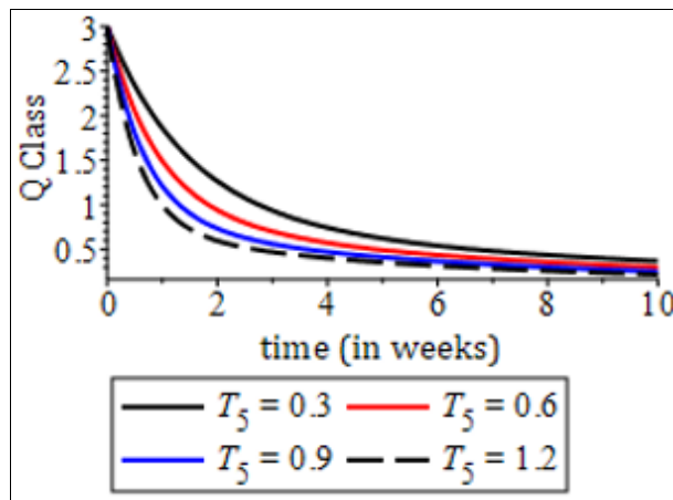
Fig 18: Impact of recovery rate with treatment to partial immunity on Quarantine class
