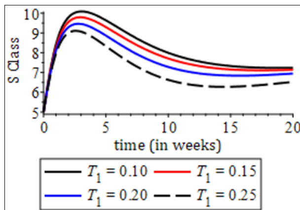
Fig 13: Effect of exposure rate of the susceptible Class
