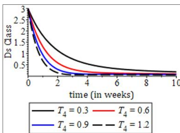
Fig 10: Impact of progression rate from symptomatically infected to not quarantined
