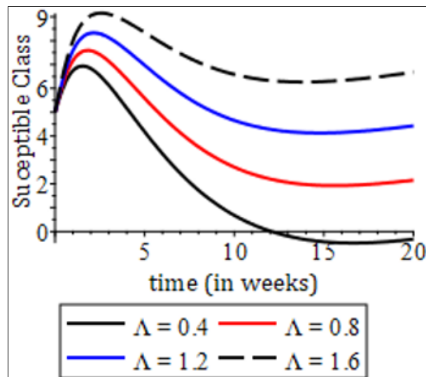
Fig 5: Impact of recruitment rate of the susceptible class
