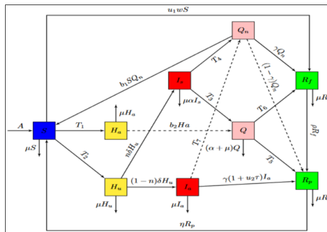
Fig 1: Compartmental model of diphtheria transmission dynamics
