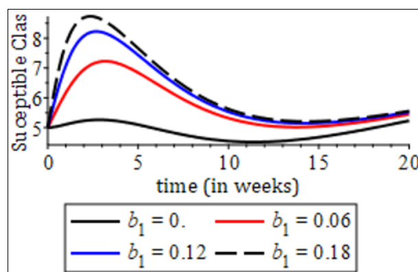
Fig 6: Effect treatment success probability on the susceptible class
