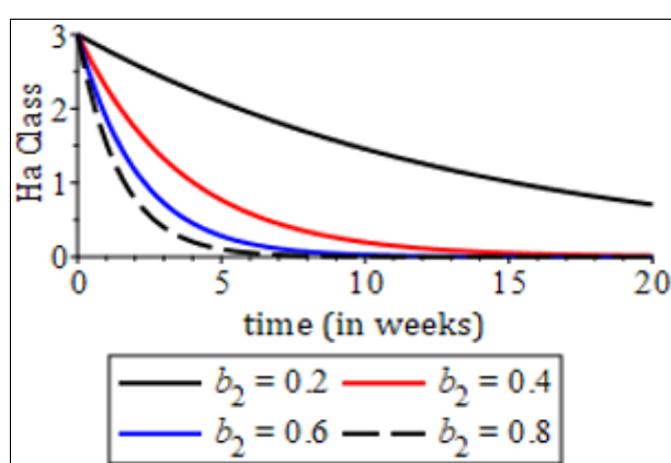
Fig 16: Impact of progression rate from exposed to quarantined
