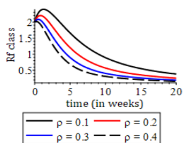
Fig 17: Impact of wanning immunity rate on Recovered with full immunity class
