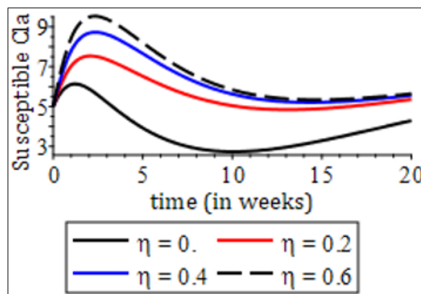
Fig 9: Impact of rate of regaining susceptibility on susceptible class
