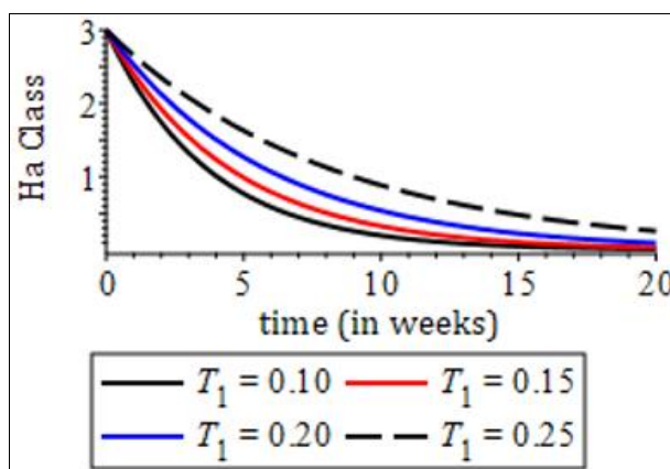
Fig 12: Effect of exposure rate on the exposed but not yet infectious class
