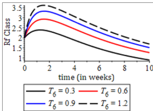
Fig 20: Impact of recovery rate with treatment to full immunity on partial recovery
