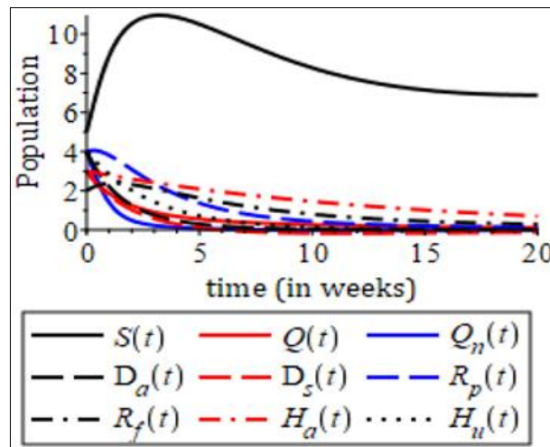
Fig 4: Model population time graph
