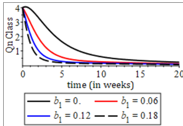
Fig 7: Effect treatment success probability on quarantined population
