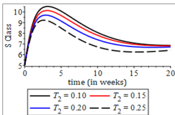
Fig 14: Impact of latency rate on the Suceptible class
