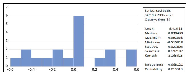
Fig 2: Normality test
